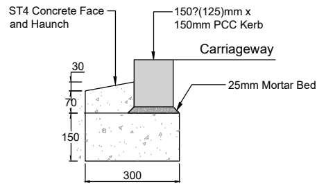
CB CHANNEL BLOCK
