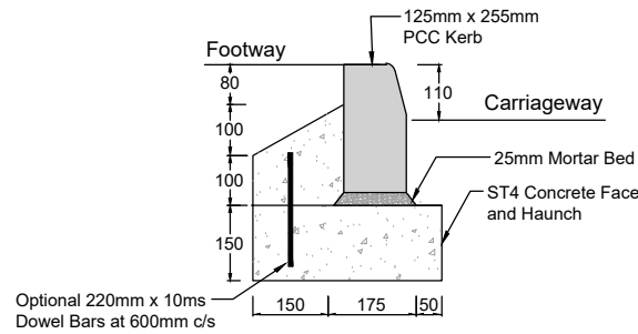
HB2 FULL HEIGHT
