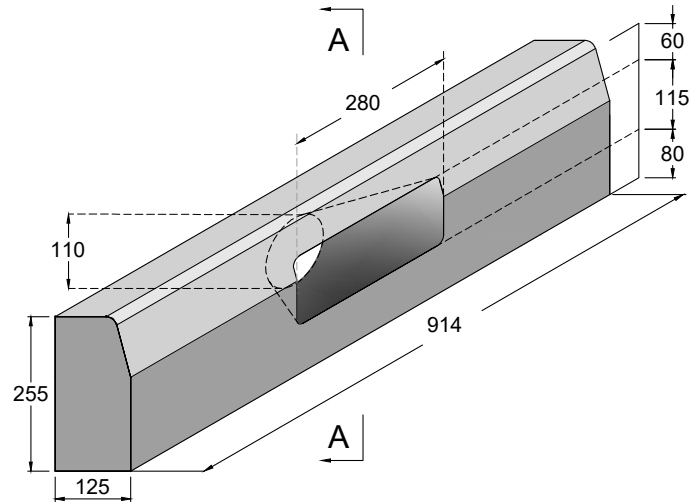
Offlet Kerb - Half Battered only
