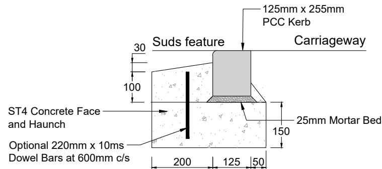
Reverse Bullnose BN2 (Flush)
