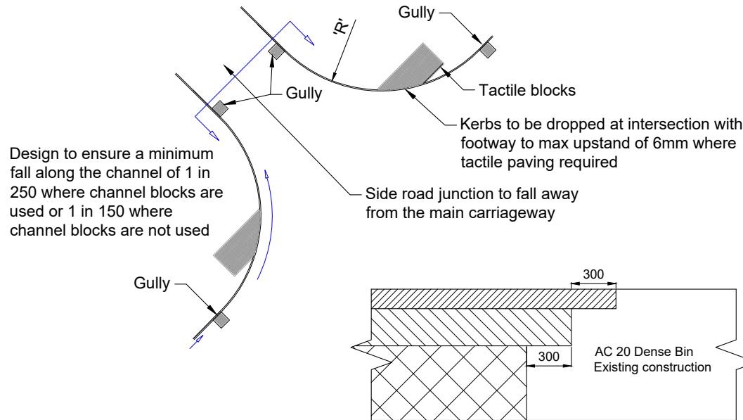
JUNCTION DETAIL WITH EXISTING CARRIAGEWAY
