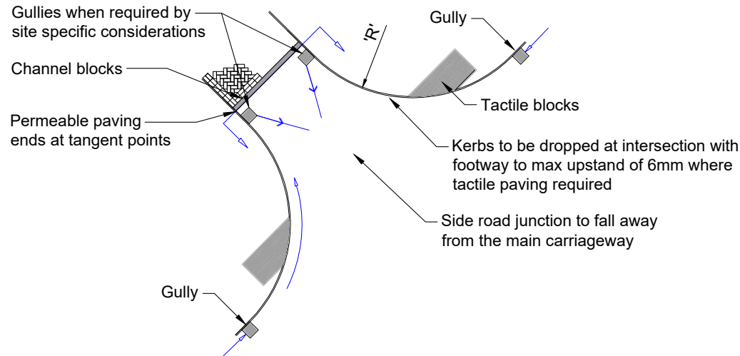
JUNCTION DETAIL WITH PERVIOUS PAVEMENT
