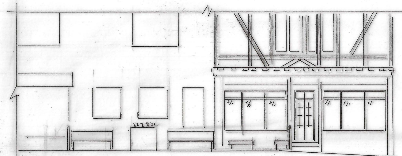
FRONT ELEVATION 1:100
